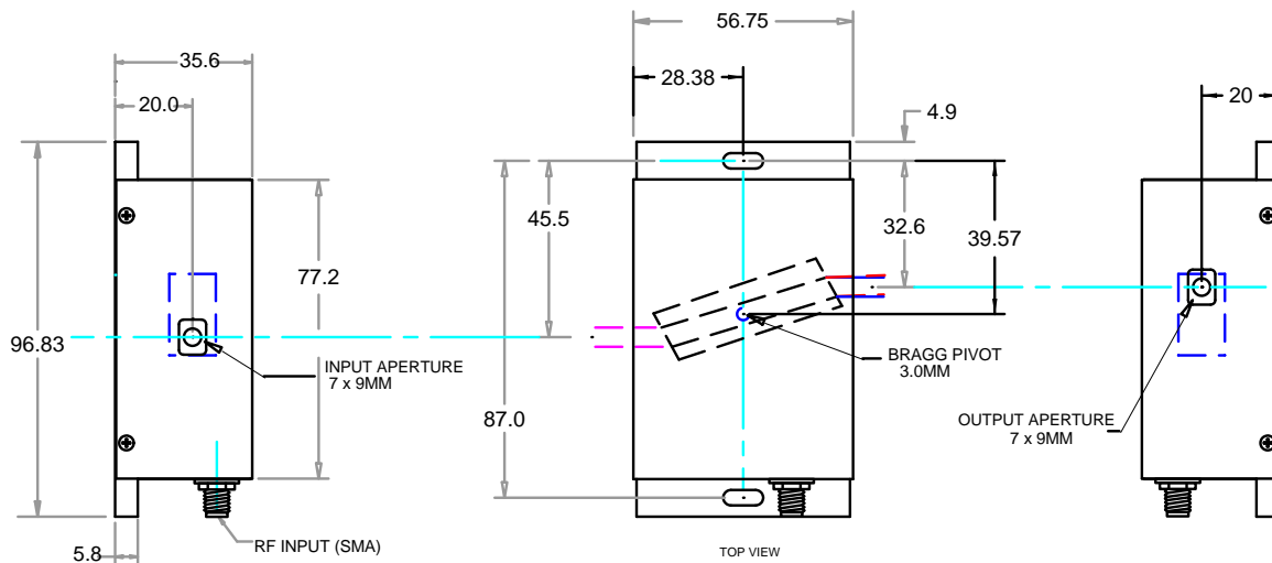
AOTF614-16 and -24 Case Dimensions, mm
